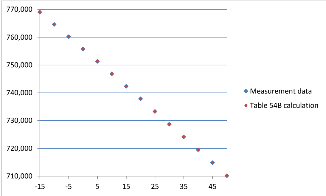
Example 1: SSR 0.11 (kg/m 3 ) 2 - Gasoline (Summer, Super)
